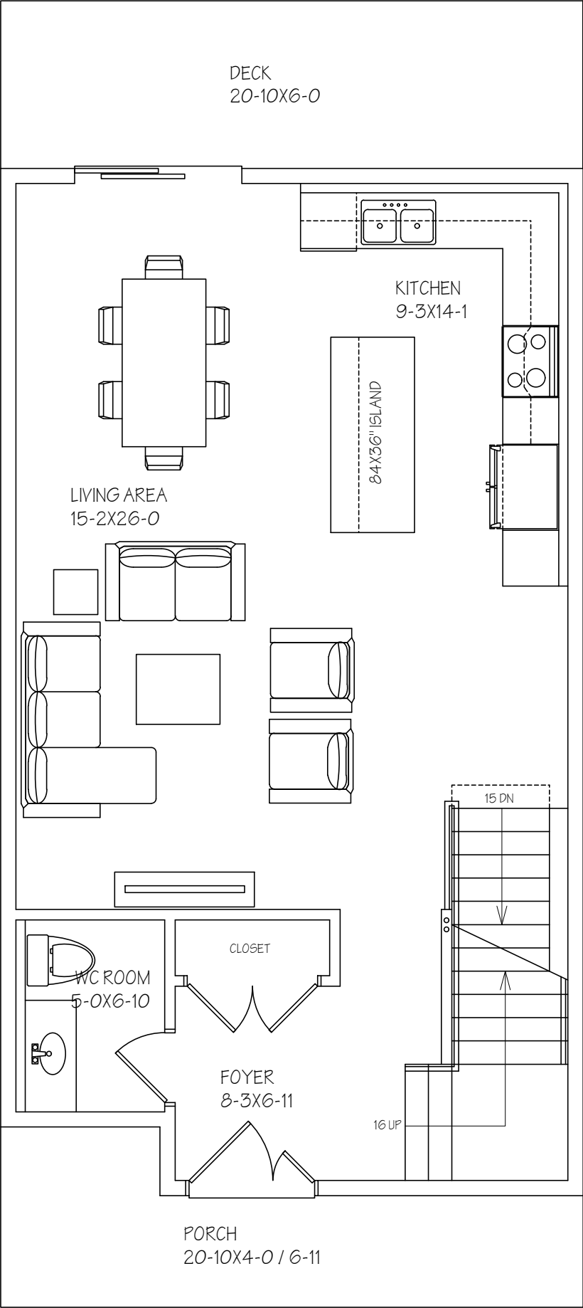
MAIN FLOOR PLAN 755.44SF
