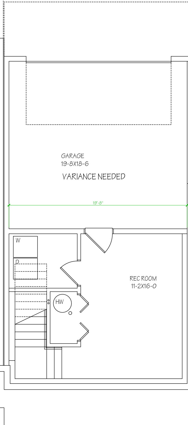
BASEMENT FLOOR PLAN 371.18SF
